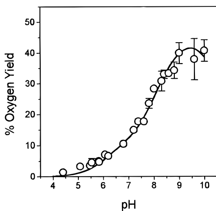
FIGURE 8. Comparison of measured (circles) and calculated (line) O_2 yields based upon Scheme 2 (adapted from ref 41).
